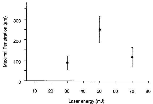
Fig. 2. Maximal penetration of fluorescent microspheres inside gelatin samples as a function of laser energy. The laser pulses were delivered via a flushing catheter with a 300 \text{ }\mu\text{m} fiber. Error bars denote the standard deviation of four samples.
