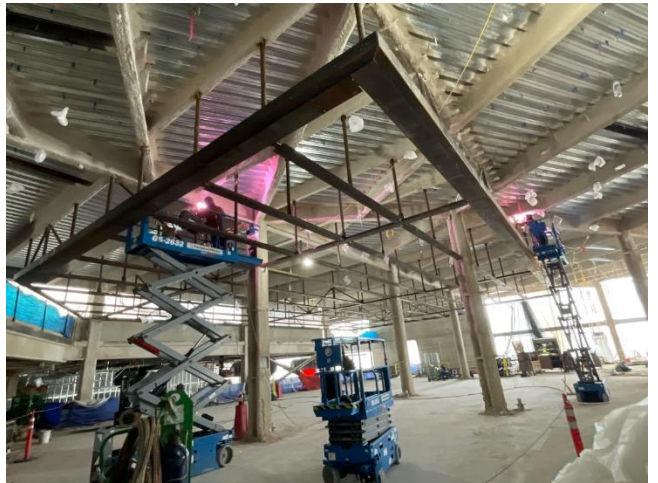
04/24/24 – Welding steel at level 2.75
